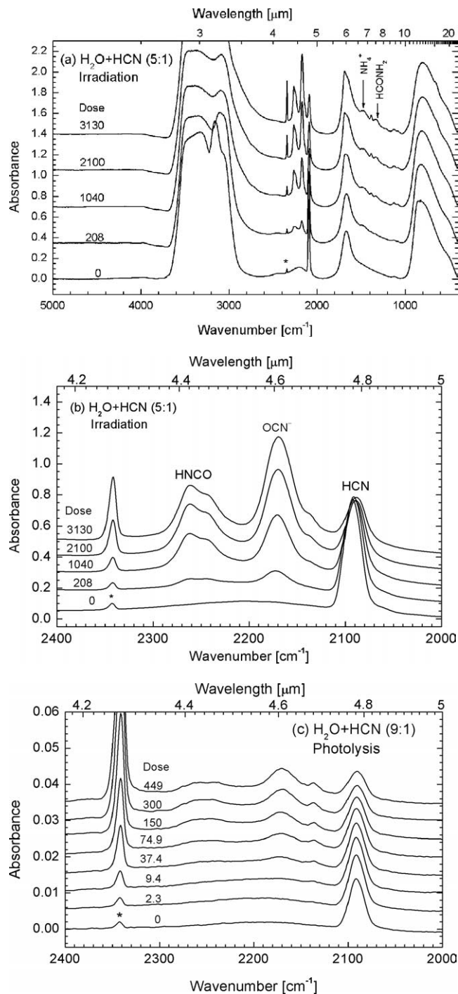
Fig. 4. (a) IR spectrum from 5000 to 400 \text{cm}^{-1} (2.0–25 \mu\text{m} ) of an \text{H}_2\text{O} + \text{HCN} (5:1) ice sample processed at 18 K by irradiation. (b) 2400–2000 \text{cm}^{-1} region of the irradiated \text{H}_2\text{O} + \text{HCN} (5:1) sample for comparison to (c) an \text{H}_2\text{O} + \text{HCN} (9:1) ice sample processed by photolysis at 18 K. Doses are in units of 10^{17} \text{eV cm}^{-2} . The absorption features of \text{CO}_2 in the initial ice deposits are marked by asterisks.
