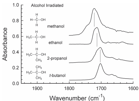
Figure 2. From top to bottom, the carbonyl ( \text{C}=\text{O} ) stretching region of the IR spectra of methanol, ethanol, 2-propanol (isopropanol), and t -butanol. Samples were irradiated at 20 K and held there while IR spectra were recorded. Spectra are offset vertically for clarity. The three vertical lines indicate positions of these products: formaldehyde ( \text{H}_2\text{CO} , 1722\text{ cm}^{-1} ), acetaldehyde ( \text{CH}_3\text{C}(\text{O})\text{H} , 1713\text{ cm}^{-1} ), and acetone ( (\text{CH}_3)_2\text{CO} , 1703\text{ cm}^{-1} ).
