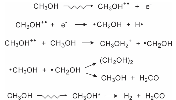
Figure 6. Reactions of irradiated CH 3 OH leading to H 2 CO, formaldehyde, among other products. Note the two reactions leading to H 2 CO: disproportionation and molecular elimination.
