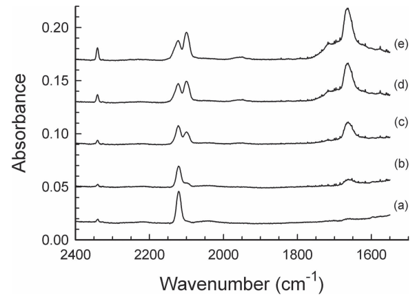
Figure 5. Expansion of Figure 4 from 2400 to 1575 cm -1 .
