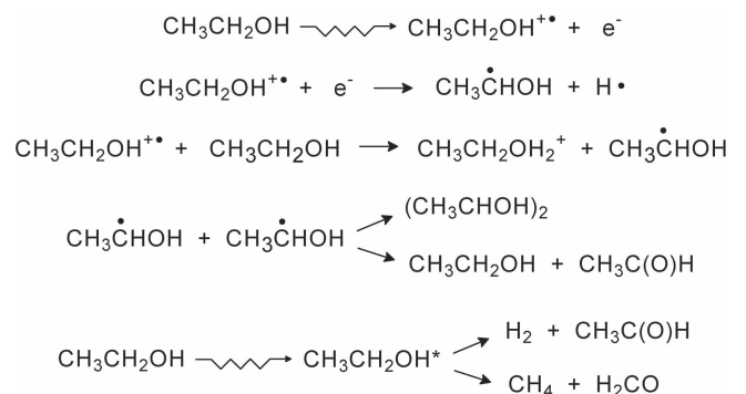
Figure 7. Reactions of irradiated CH 3 CH 2 OH leading to CH 3 C(O)H and H 2 CO, acetaldehyde and formaldehyde, respectively, among other products. Note the two reactions leading to CH 3 C(O)H, disproportionation and molecular elimination, and the one reaction leading to H 2 CO.
